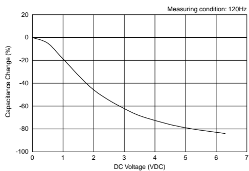
High Dielectric Constant Type: GRM31CR60J107ME39
