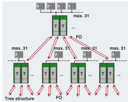
Redundant structure
