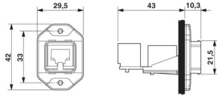
Push-Pull SCRJ panel mounting frame
