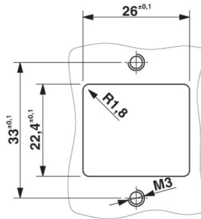
Panel cutout
