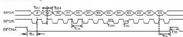
Figure9 SPI write timing
