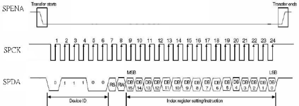
Figure10 SPI timing
