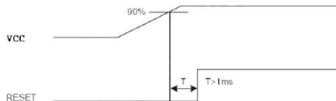
Reset timing
