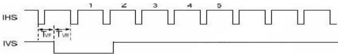
Figure7 IHS and IVS Timing Waveform
