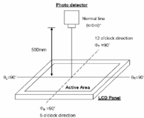
Fig. 8-2 Optical measurement system setup
