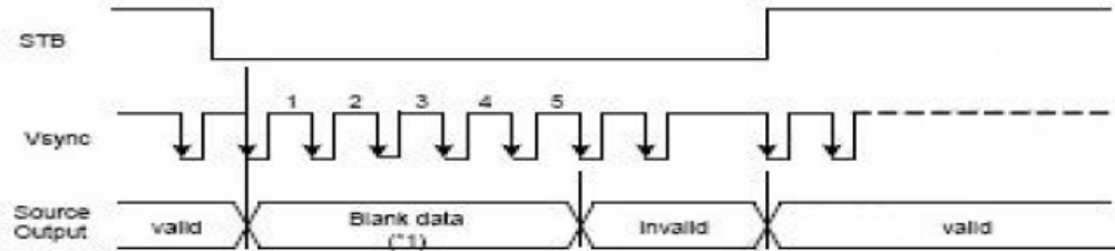
Figure5 Standby ON / OFF Control
