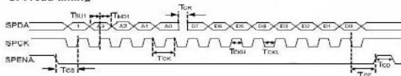
Figure8 SPI read timing
