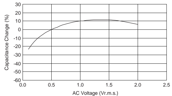
[AC Voltage Characteristics]
