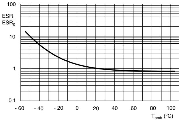
Fig.8 Typical multiplier of ESR as a function of temperature at 100 Hz ESR_0 = typical ESR at 20 °C, 100 Hz
