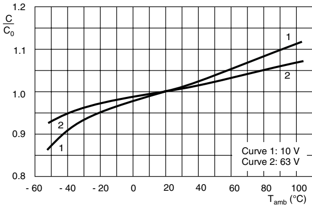
Fig.6 Typical multiplier of capacitance as a function of temperature at 100 Hz C_0 = capacitance at 20 °C, 100 Hz
