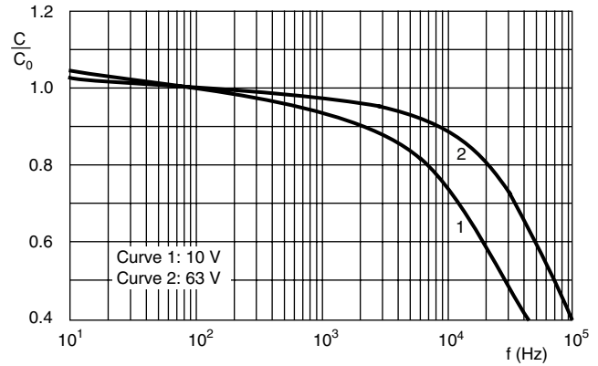
Fig.7 Typical multiplier of capacitance as a function of frequency at 20 °C C_0 = typical capacitance at 20 °C, 100 Hz
