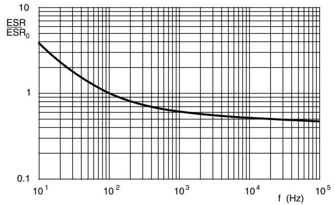
Fig.9 Typical multiplier ESR as a function of frequency at 20 °C ESR_0 = typical ESR at 20 °C, 100 Hz
