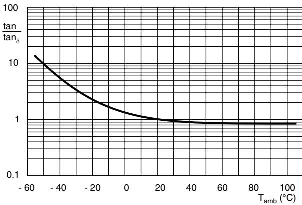
Fig.10 Typical multiplier of dissipation factor \tan \delta as a function of temperature at 20 °C at 100 Hz \tan \delta_0 = typical \tan \delta at 20 °C, 100 Hz
