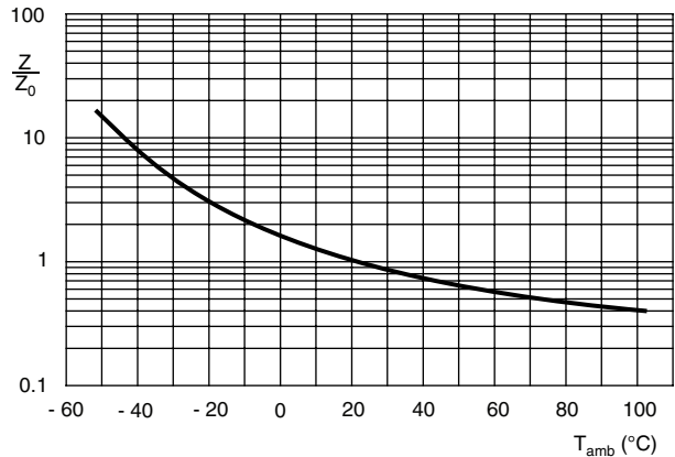
Fig.11 Typical multiplier of impedance Z as a function of temperature at 100 kHz Z_0 = typical impedance Z at 20 °C, 100 kHz
