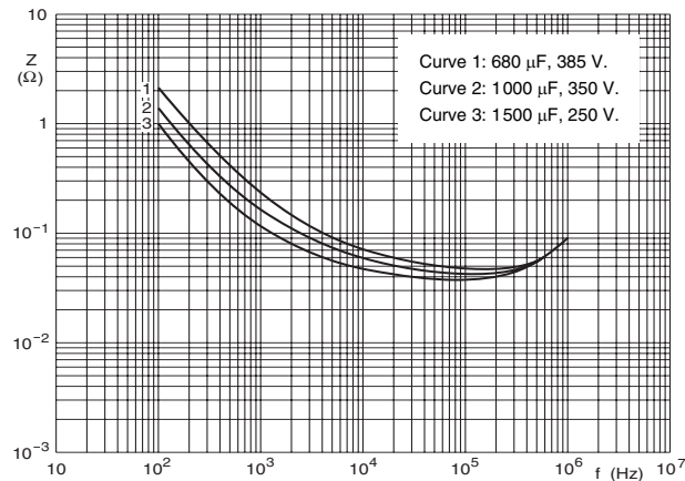
Case \varnothing D \times L = 50 \times 105 mm.
