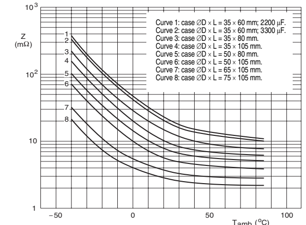
Z at 20 kHz and U_R = 63 V.
