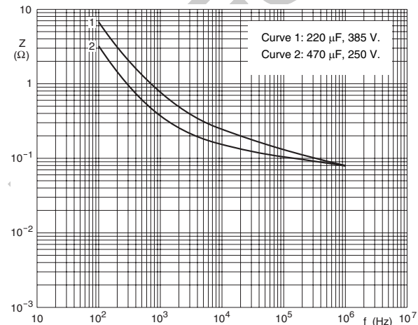
Case \varnothing D \times L = 35 \times 80 mm. T_{amb} = 20 °C.
