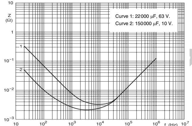
Case \varnothing D \times L = 65 \times 105 mm. T_{amb} = 20 °C.
