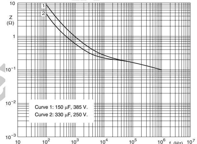
Case \varnothing D \times L = 35 \times 60 mm. T_{amb} = 20 °C.
