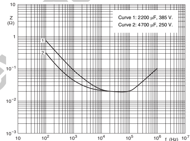
Case \varnothing D \times L = 75 \times 105 mm.
