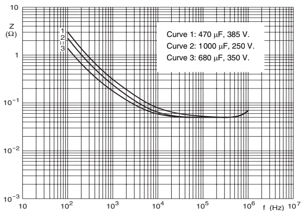
Case \varnothing D \times L = 50 \times 80 mm.
