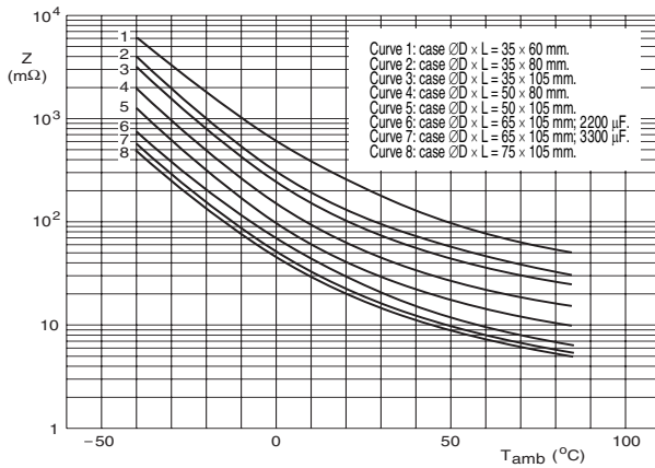
Fig.9 Typical impedance as a function of temperature.
