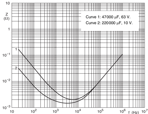
Case \varnothing D \times L = 75 \times 105 mm. T_{amb} = 20 °C.
