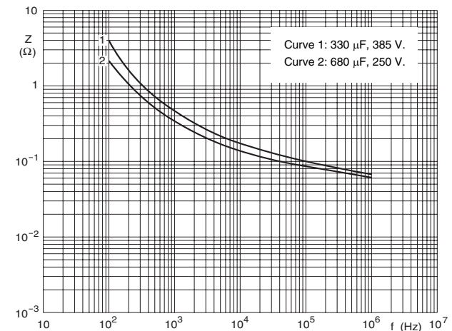
Case \varnothing D \times L = 35 \times 105 mm. T_{amb} = 20 °C.
