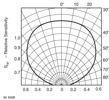
Figure 8. Relative Radiant Sensitivity vs. Angular Displacement
