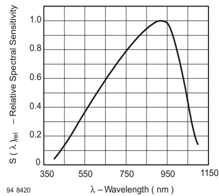
Figure 7. Relative Spectral Sensitivity vs. Wavelength
