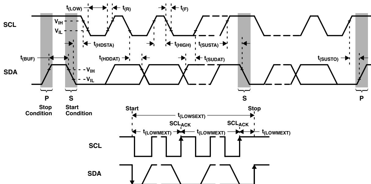
Figure 2. Timing Diagrams
