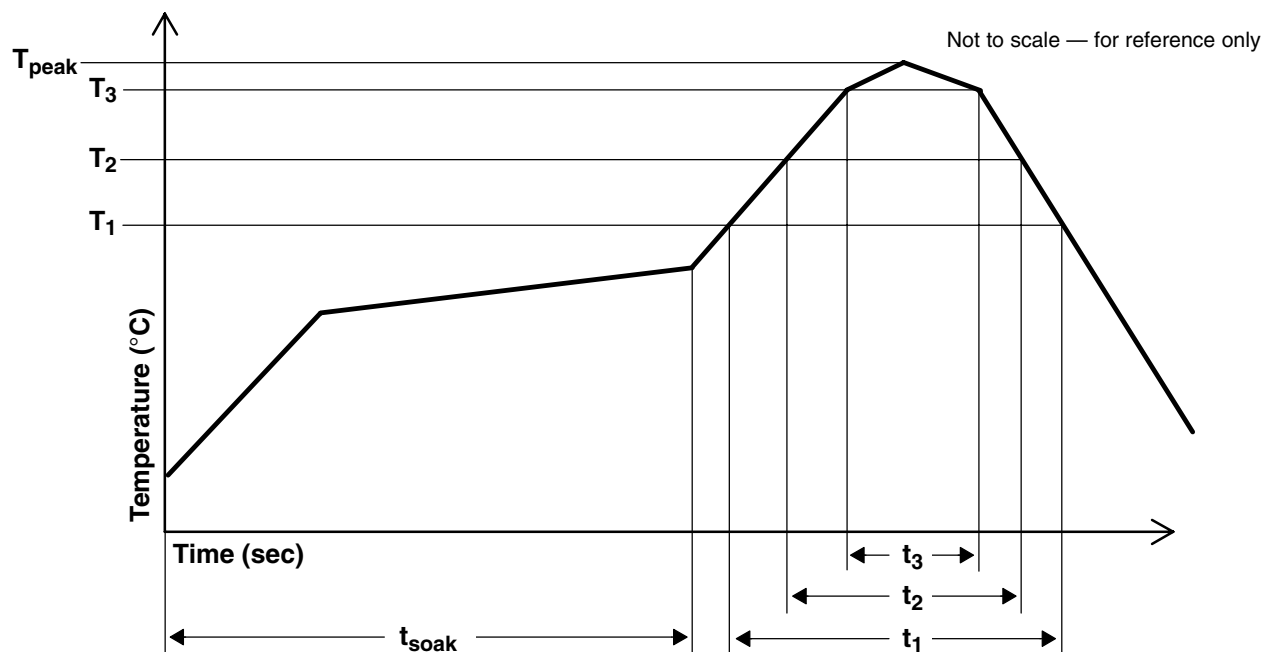
Figure 30. TCS3404/TCS3414 Solder Reflow Profile Graph
