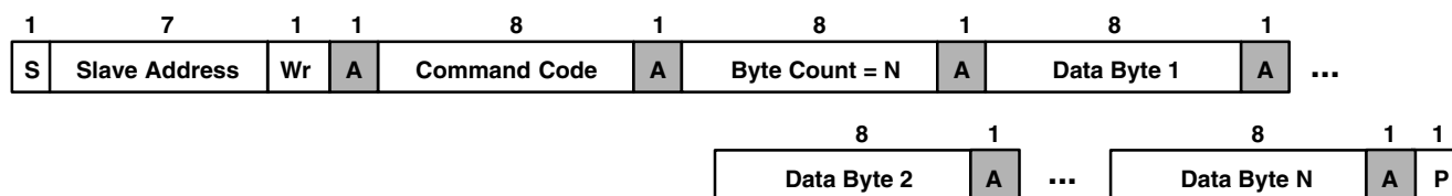
Figure 18. SMBus Block Write or I²C Write Protocols
