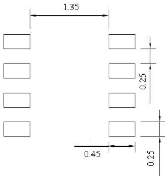
PCB Soldering Pad
