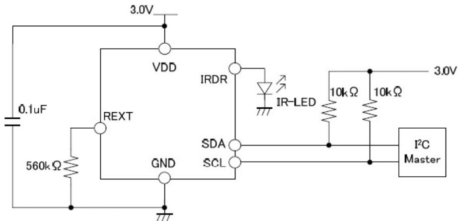
Figure 2. APS-12D-1-02/TR8 Typical Application Circuit
