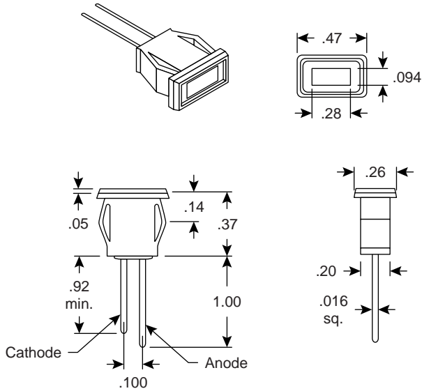
Dimensions (In.)
