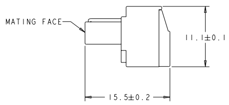
796693-3 AS SHOWN
