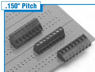
.150" Pitch ELVM . . . . . Page 60 12A / 300V
