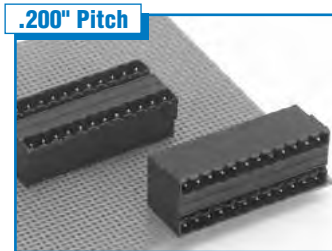
.200" Pitch ELFA 2-Tier Aligned H/V . . . Page 49 15A / 300V
