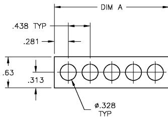
RECOMMENDED PANEL LAYOUT
