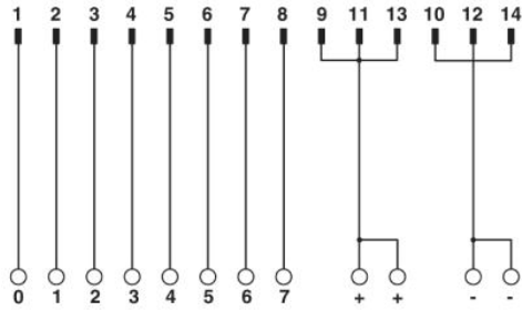
UM 45-FLK14/PLC connection scheme
