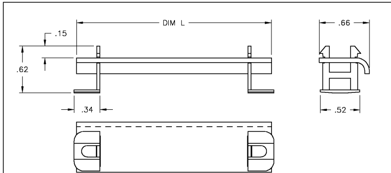
ASSEMBLED VIEW
