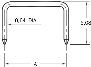
3360-X-14-XX-00-00-08-0 Shorting Jumper
