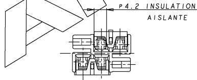
DETALLE CON BISAGRA CERRADA HOUSING WITH CLOSED FLAP
