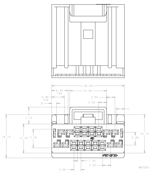
638116-1 SHOWN KEY A CONFIGURATION
