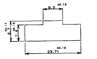
パネル取付穴寸法 FIG 1 (RECOMMENDED PANEL OPENING DIMENSION)
