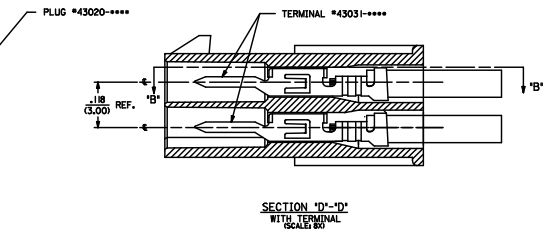
MATED MICRO-FIT CONNECTOR
