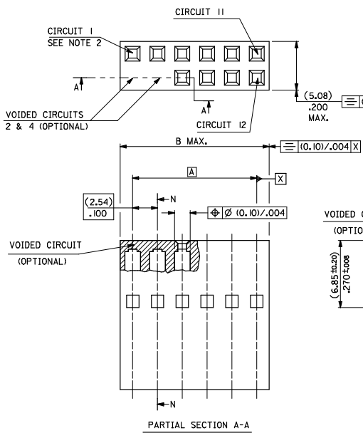
NO POLARISING BUTTON VERSION (90143-0** VERSION)
