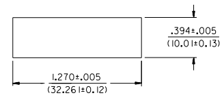
RECOMMENDED HOLE CUTOUT
