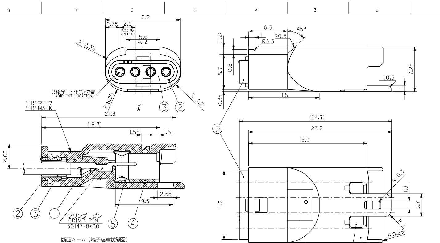
断面A-A (端子装着状態図) SECT.A-A (TERM.ASSEMBLY DRAWING)
