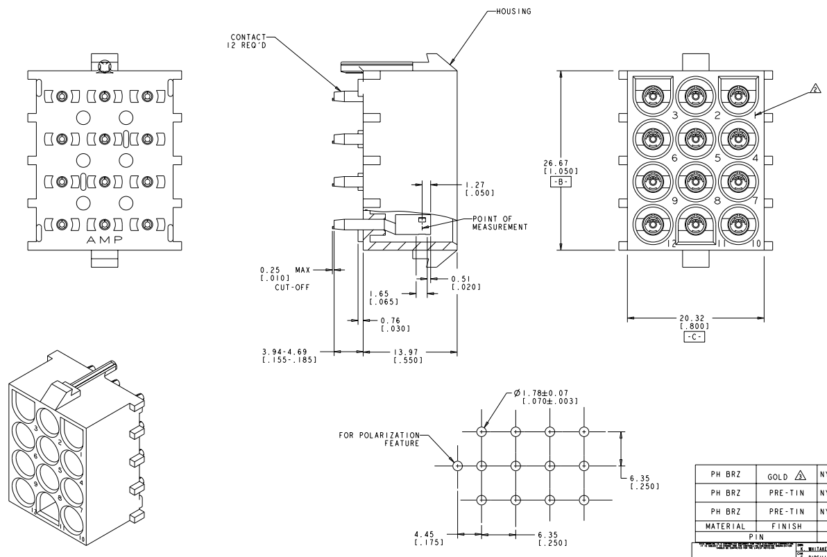
3 DIMENSIONAL MODEL SCALE 4:1
