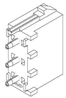
3-DIMENSIONAL MODEL NTS
