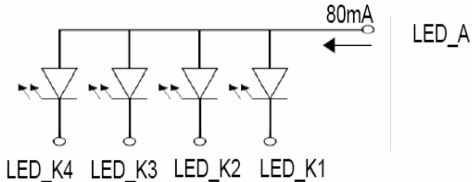
* 1 Backlight LED Circuit:
