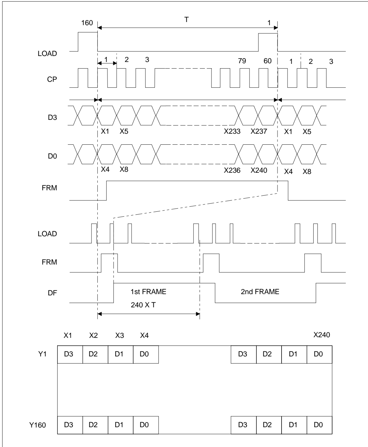
Signal Timing (2)
