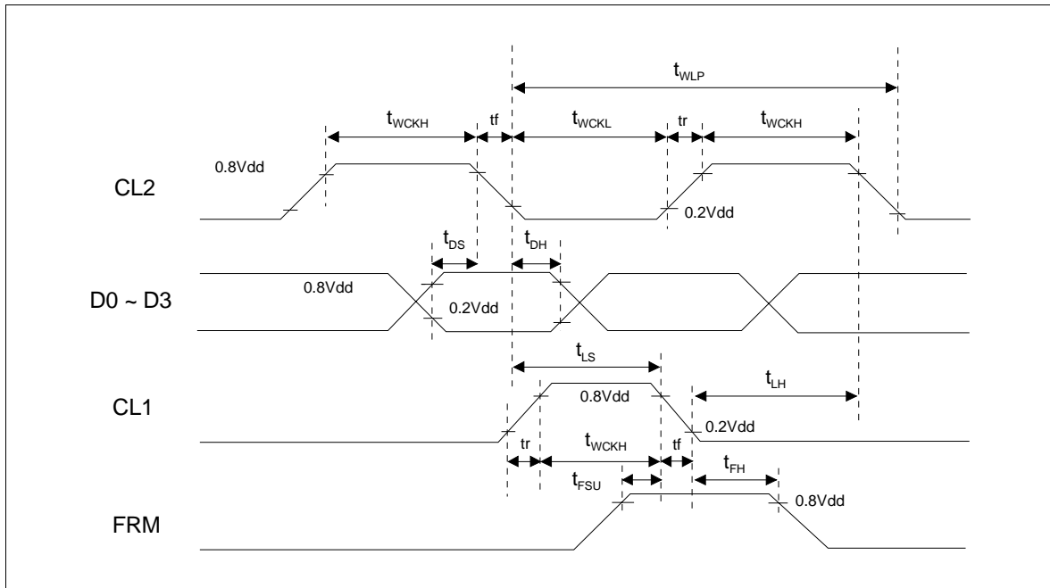
Signal Timing(1)
