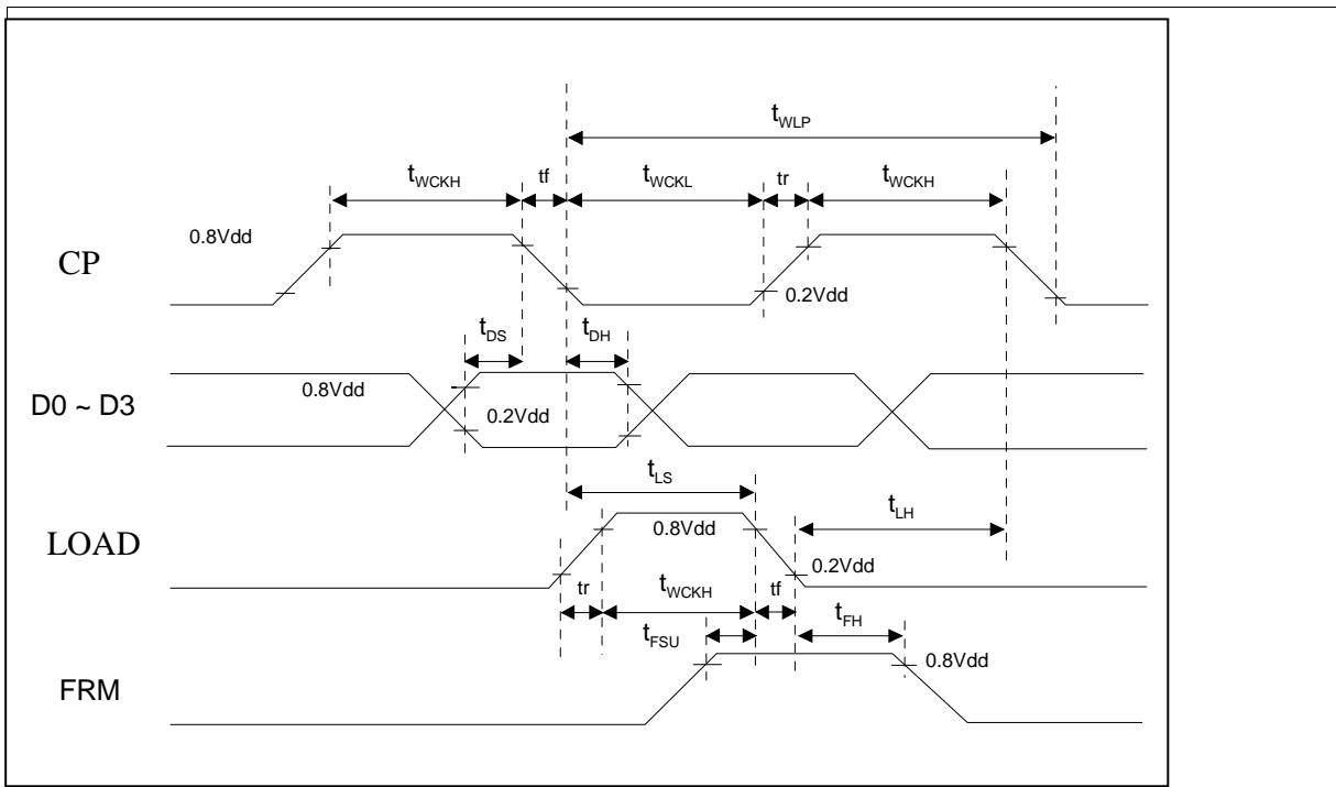
Signal Timing(1)
