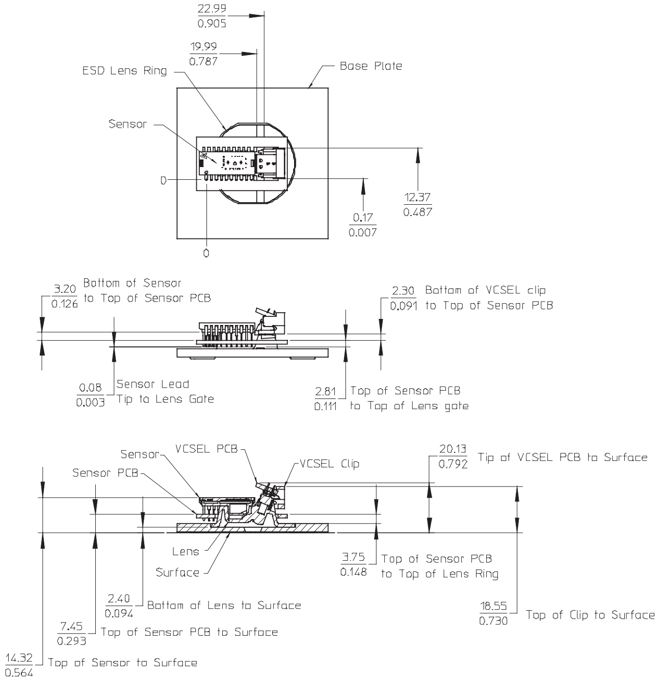
Figure 1. Assembly drawing of ADNB-6001-EV (top, front and cross-sectional view)
