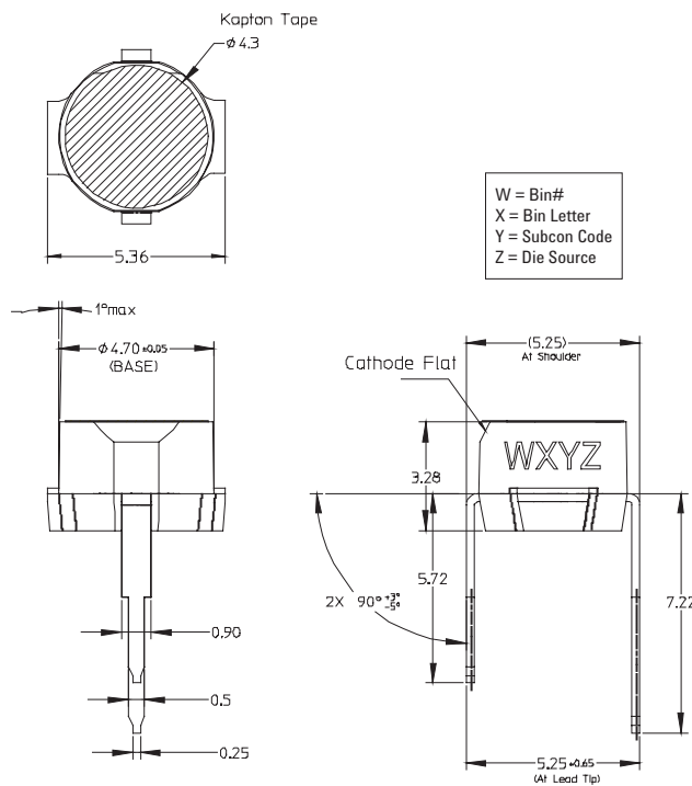
Figure 31. Outline Drawing for ADNV-6340 VCSEL
