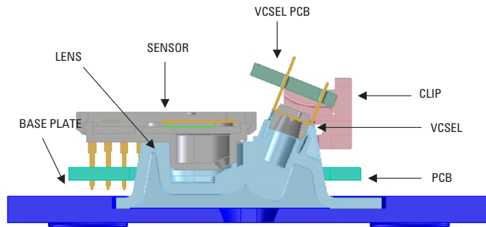
Figure 4. Cross section of PCB assembly
