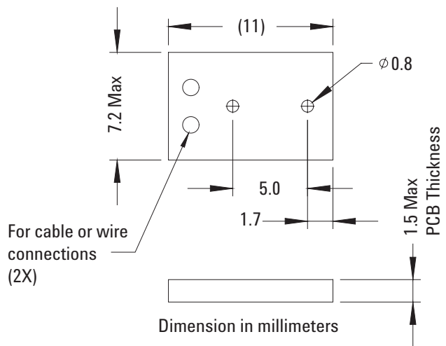
Figure 32. Suggested ADNV-6340 PCB Mounting Guide
