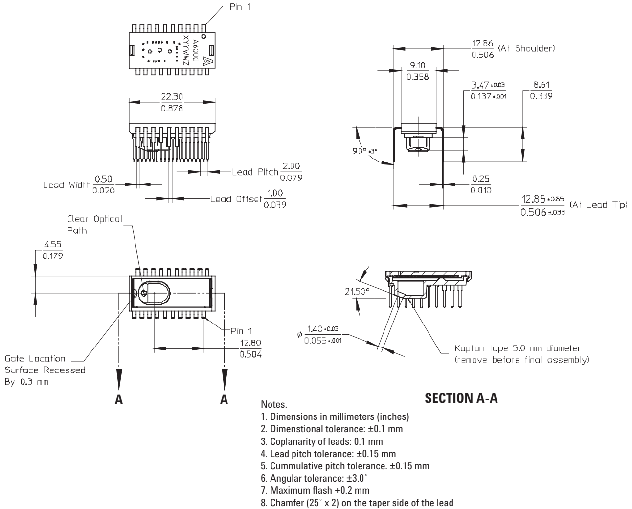
Figure 8. Package outline drawing
