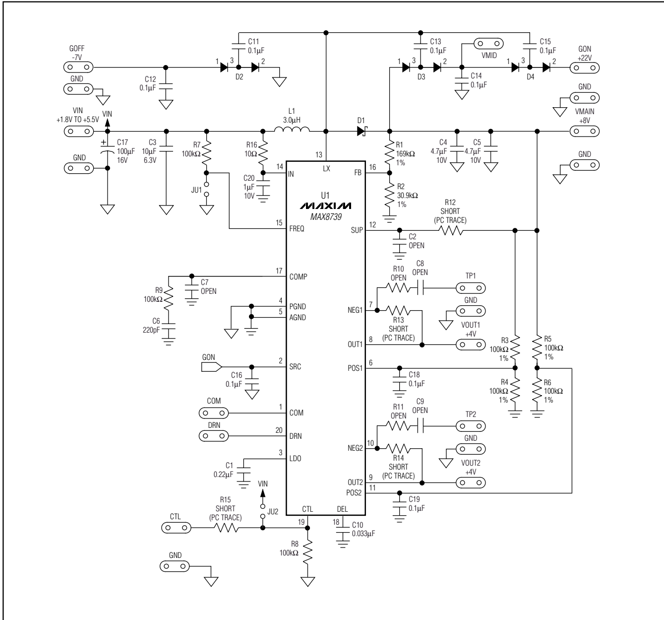
Figure 1. MAX8739 EV Kit Schematic
