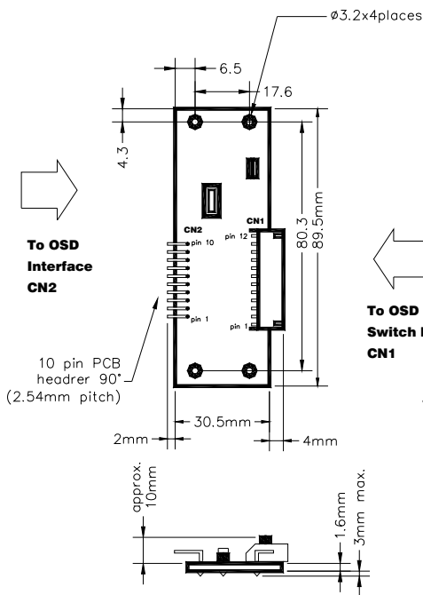
Membrane Interface Board: P/N:416100120-3
