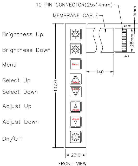
Membrane Switch: P/N:356301021-3
