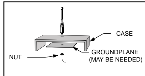
figure 13: Remote Groundplane
