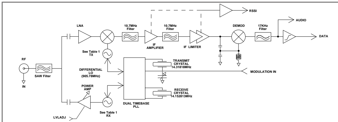
Figure 7: SC-S Series Block Diagram
