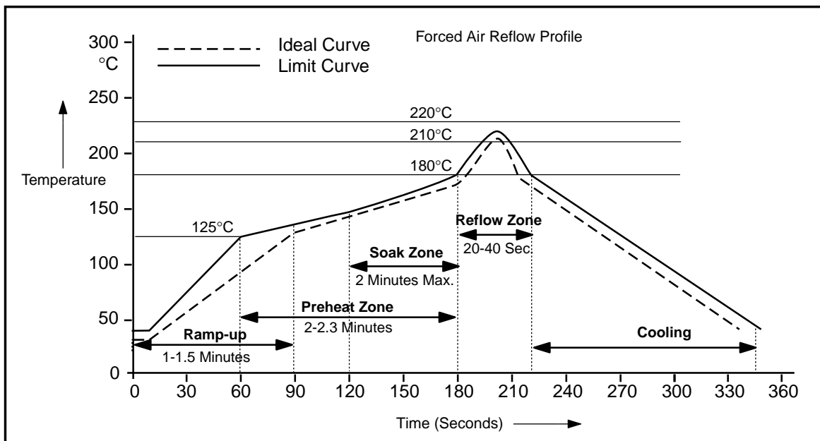
figure 15: Maximum reflow profile
