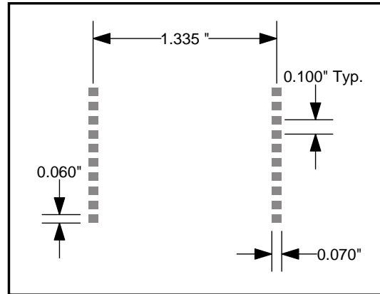
Figure 6: Recommended pad layout
