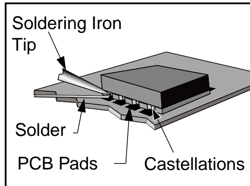
Figure 14: Soldering Technique
