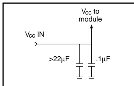
Figure 8: Suggested supply filter
