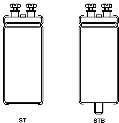
Fig.1 Component outlines
