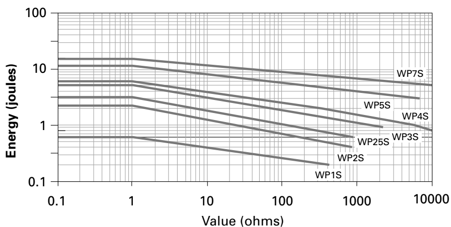
WP-S Short Pulse Energy Capacity
