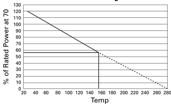
W31 Series Derating Curve
