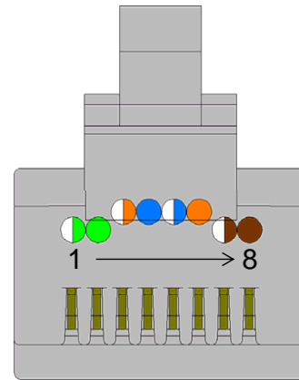
CAT6a Plug (TM31P-TM-88P)
