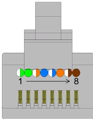
CAT6 Plug (TM21DP-TM-88P)
