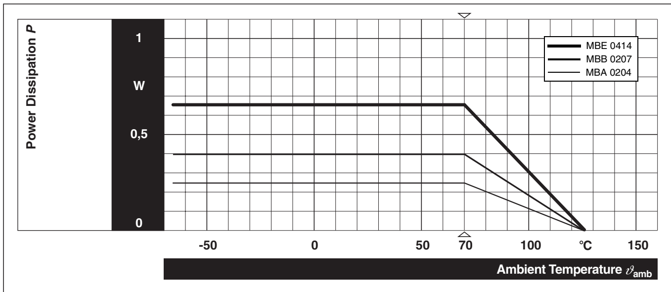
Fig.2 Derating, long term operation.
