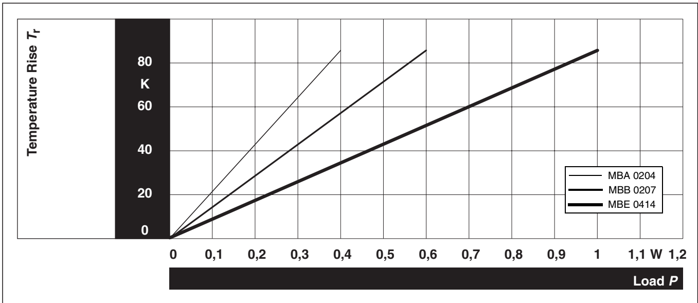
Fig.3 Rise of the surface temperature.
