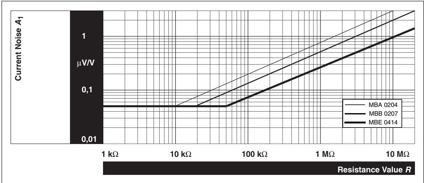
Fig.9 Current noise A_1 in accordance with IEC 60195.
