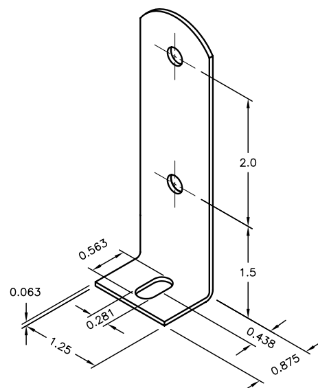
Brackets Dimensions
