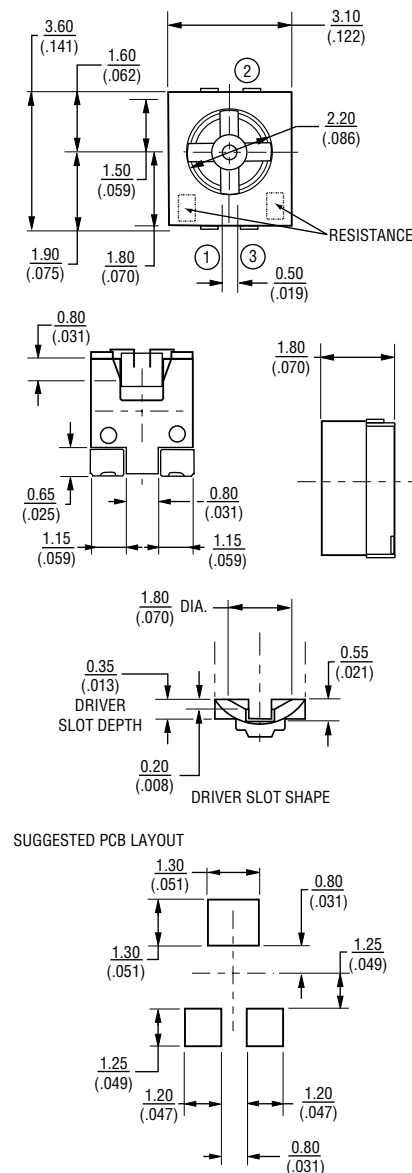
DIMENSIONS: MM/(INCHES)
