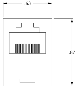
RJ45 JACK (8 X 8)
