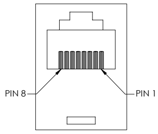
RJ45 JACK (8 X 8)
