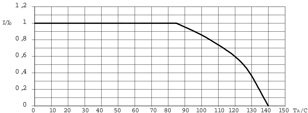
B82464-XXXX-X: current derating versus ambient temperature
