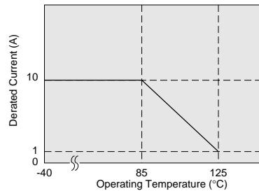
Derating
