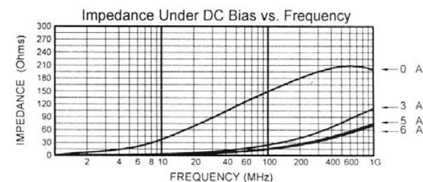
MLB-453215-0150PW
