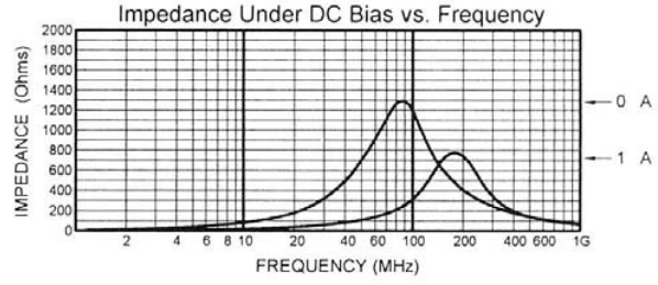
MLB-321611-1200PL
