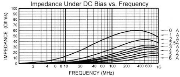
MLB-321611-0050PW
