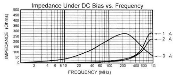
MLB-160808-0220PN
