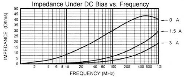
MLB-160808-0030PQ
