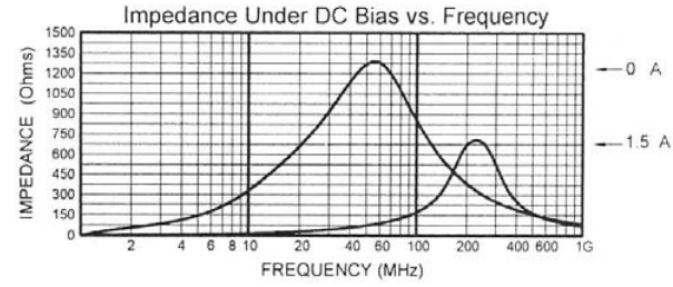
MLB-451616-0850PM
