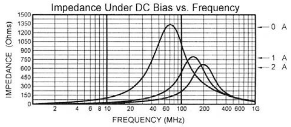
MLB-322513-1000PN
