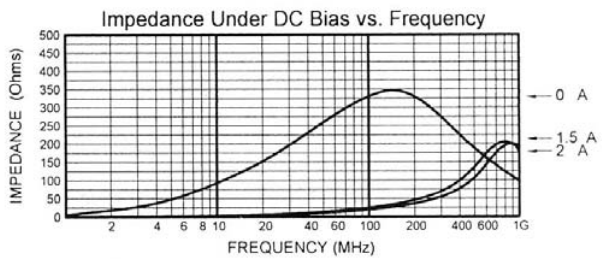
MLB-201209-0330PN
