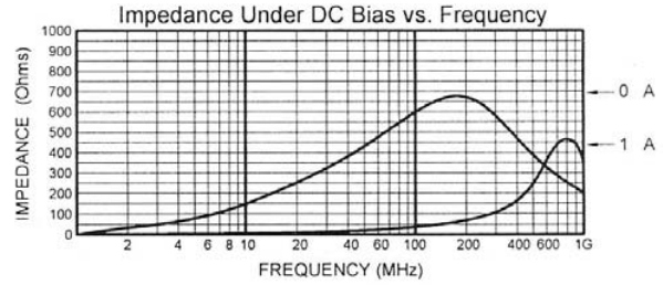
MLB-160808-0600PL
