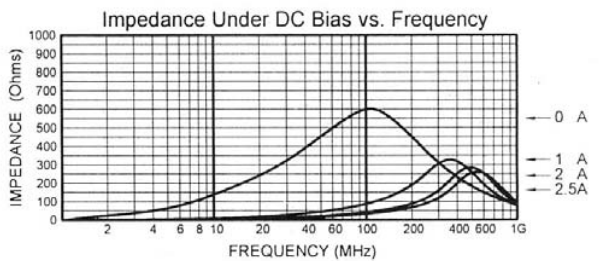
MLB-321611-0600PP
