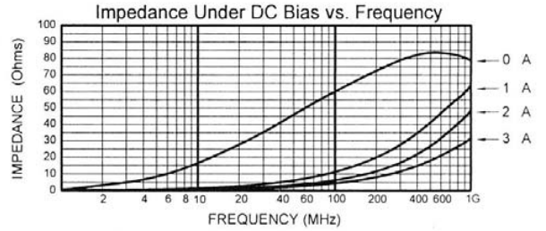
MLB-160808-0060PQ
