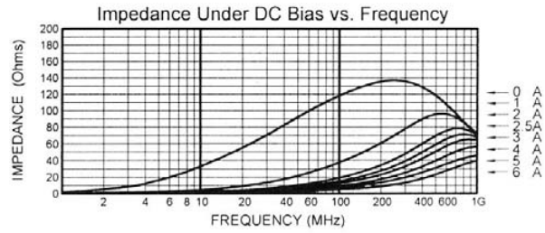
MLB-321611-0120PW
