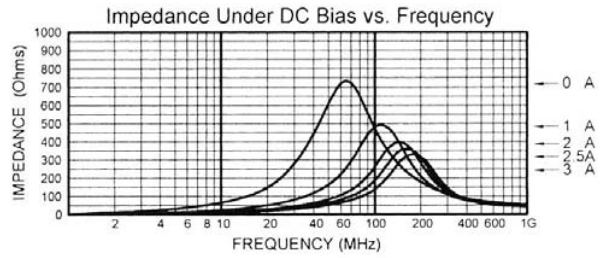
MLB-453215-0600PQ
