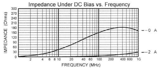
MLB-321611-0150PN
