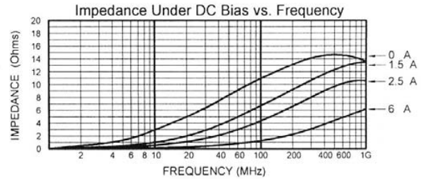
MLB-201209-0011PW
