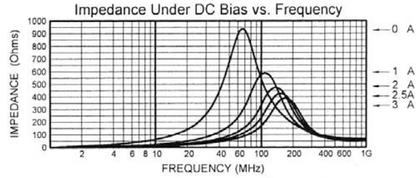
MLB-453215-0680PQ
