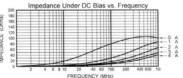
MLB-321611-0080PR
