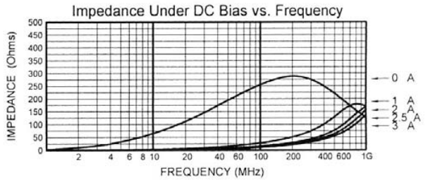
MLB-201209-0250PQ
