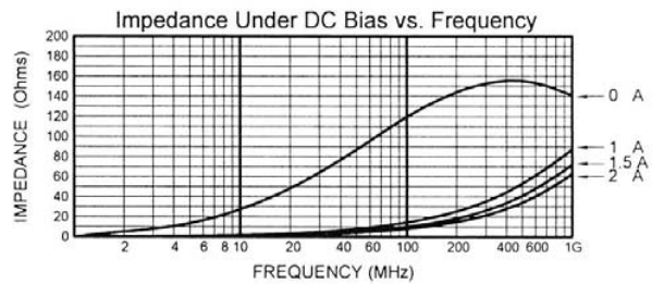
MLB-160808-0120PP
