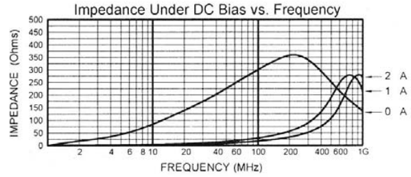
MLB-160808-0300PN
