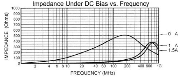
MLB-160808-0450PM
