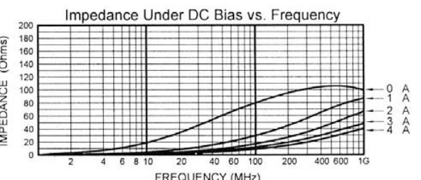
MLB-321611-0090PQ
