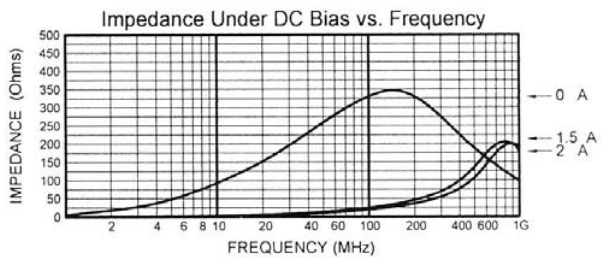
MLB-201209-0600PN
