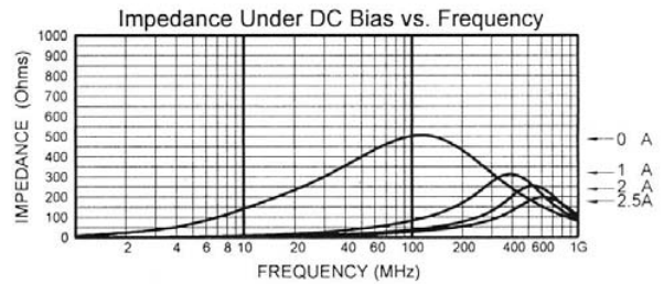
MLB-321611-0500PP
