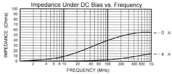
MLB-201209-0040PR
