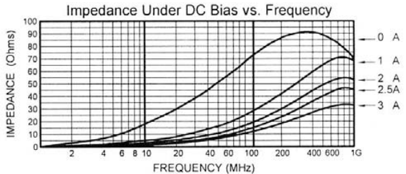
MLB-321611-0075PQ
