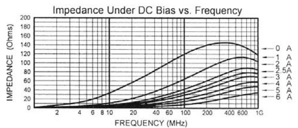
MLB-453215-0120PW
