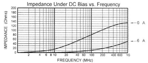
MLB-453215-0080PW
