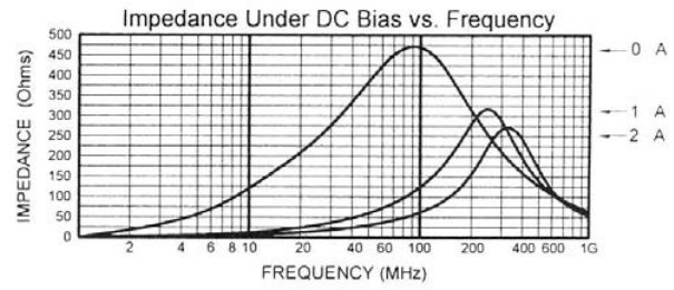
MLB-451616-0470PN
