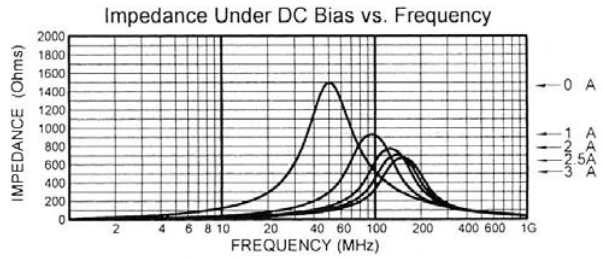
MLB-453215-1300PQ
