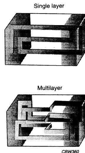
Fig.2 Internal structure of multilayer suppressors.
