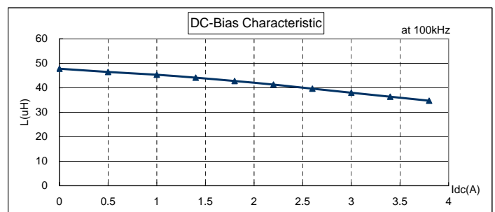
DC-Bias Characteristic
