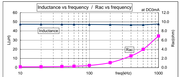
Inductance vs frequency
