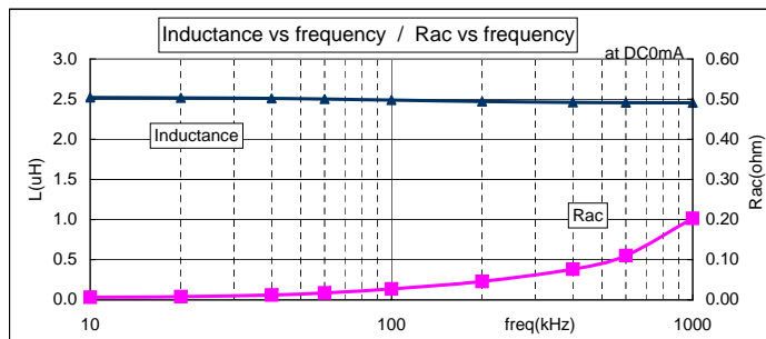
Inductance vs frequency
