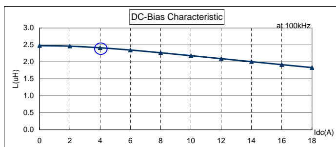
DC-Bias Characteristic
