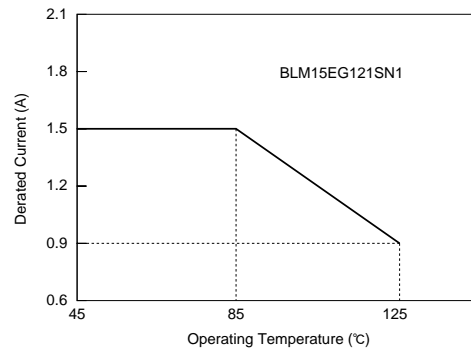
[Derating]
