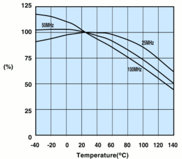
Measured on a 2644000301 using the HP4291A.
