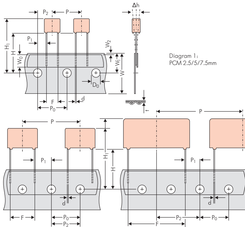
Diagram 2: PCM 10/15 mm
