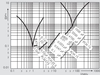
Impedance change with frequency (general guide)
